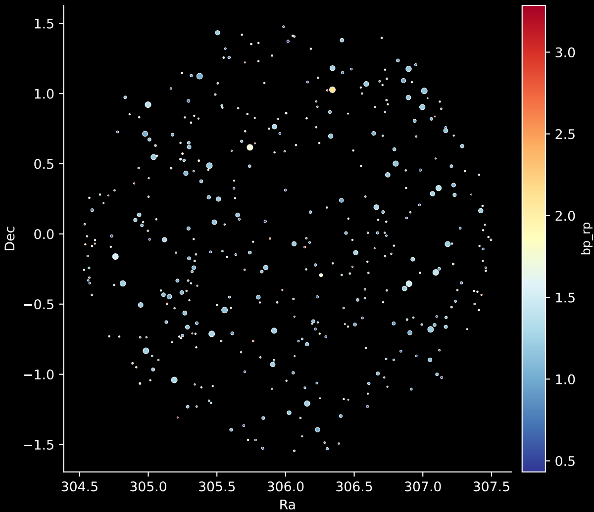
APOGEE DR17 Field: [330+60] Stars: 405
