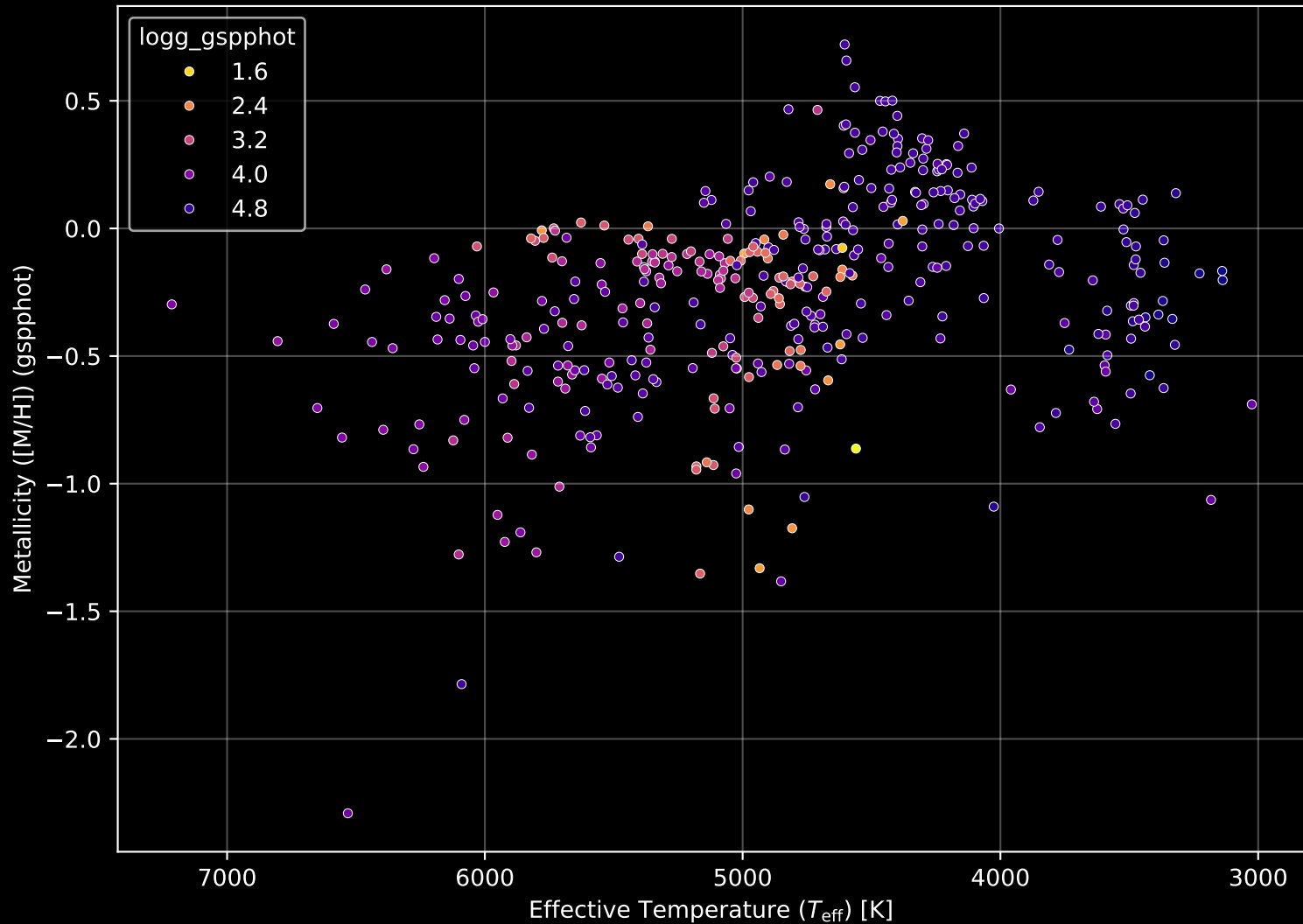
APOGEE DR17 Field: [330+60] Stellar Population Parameters (n= 405)
