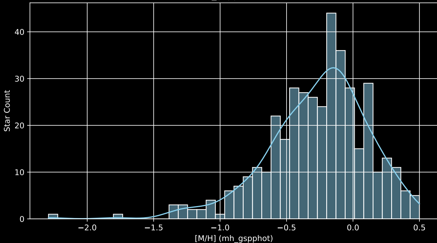
APOGEE DR17 Field: [330+60 [M/H] (mh_gspphot) (n= 401)
