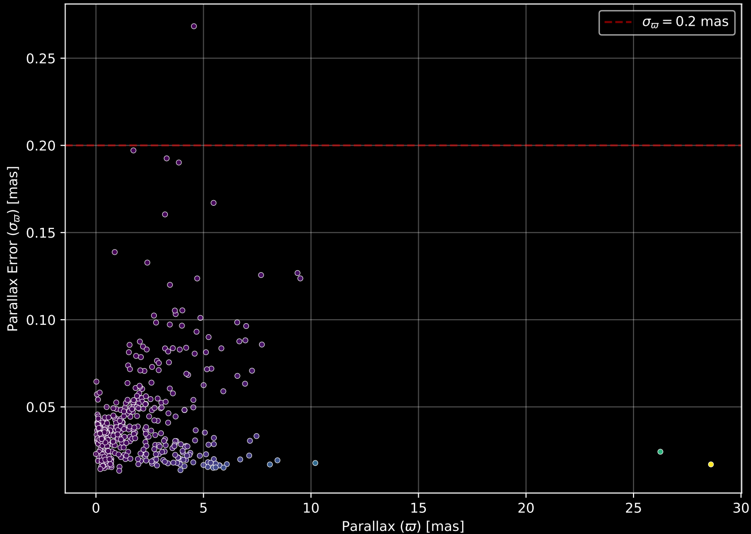
APOGEE DR17 Field: [330+60] Parallax Quality (n= 405)
