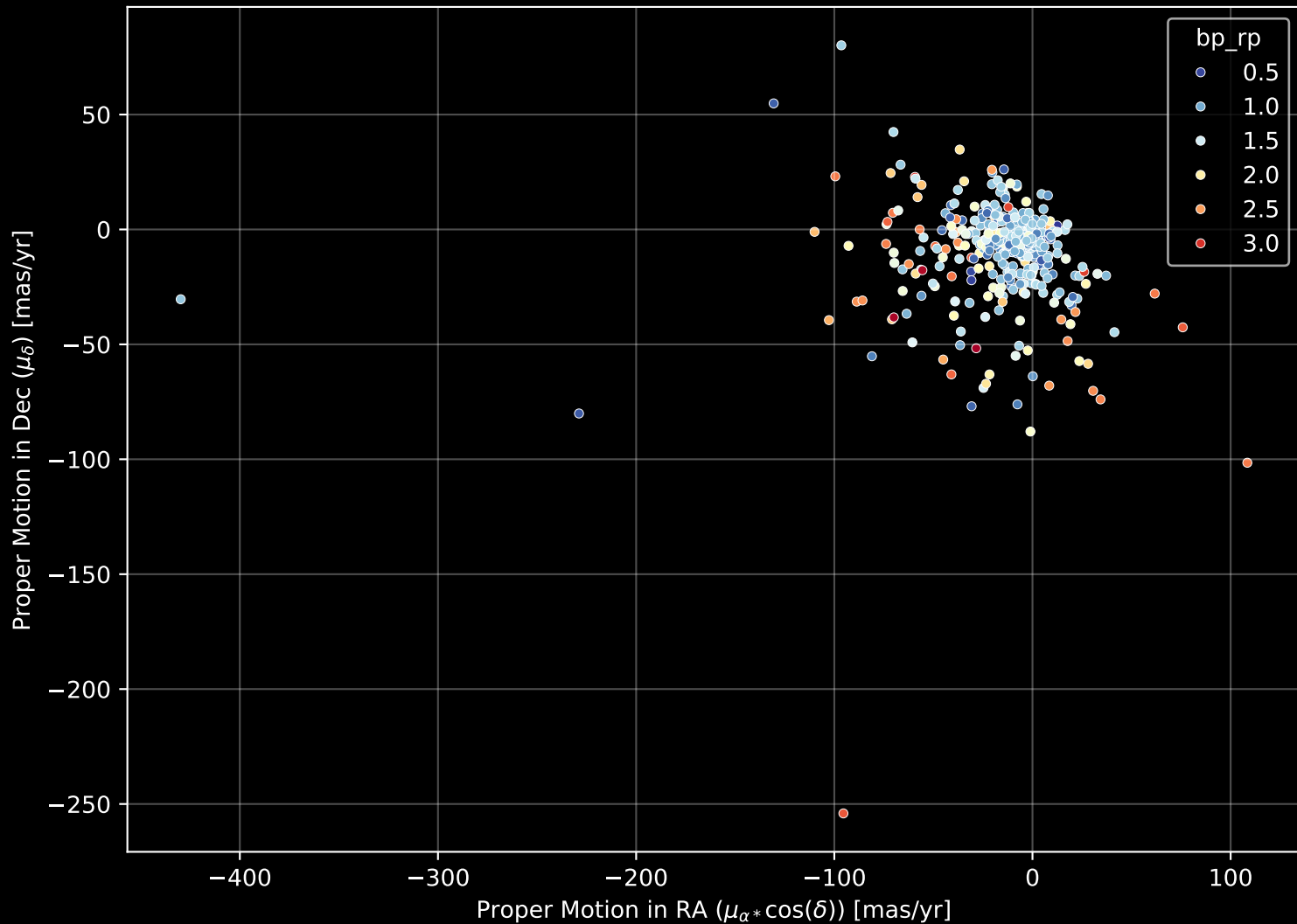
APOGEE DR17 Field: [330+60] Proper Motion Diagram (n= 405)
