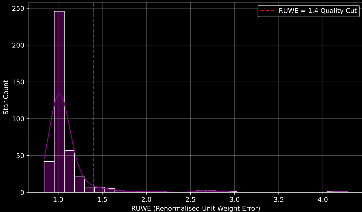
GAPOGEE DR17 Field [330+60] RUWE Distribution (n= 397)
