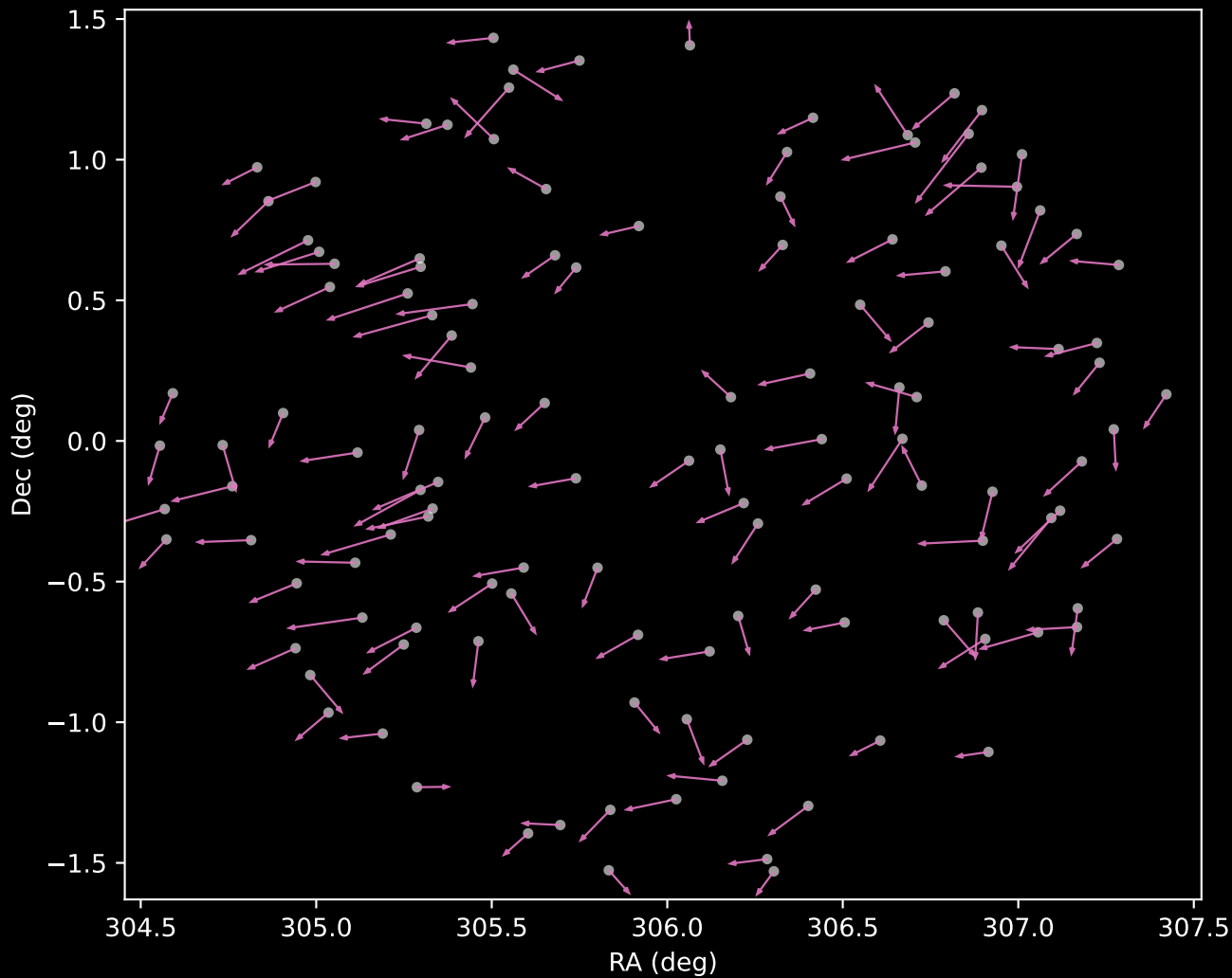
APOGEE DR17 Cluster 12 Proper Motion Vectors (n=127)
