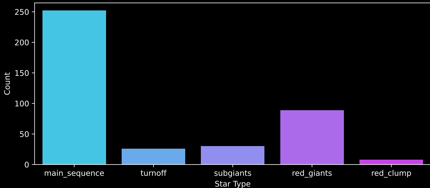
APOGEE DR17 Field: [330+60] Count plot of Star Type
